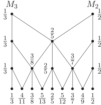
FIGURE 2. Bratteli diagram of \mathfrak{A}/\mathcal{J}_2
