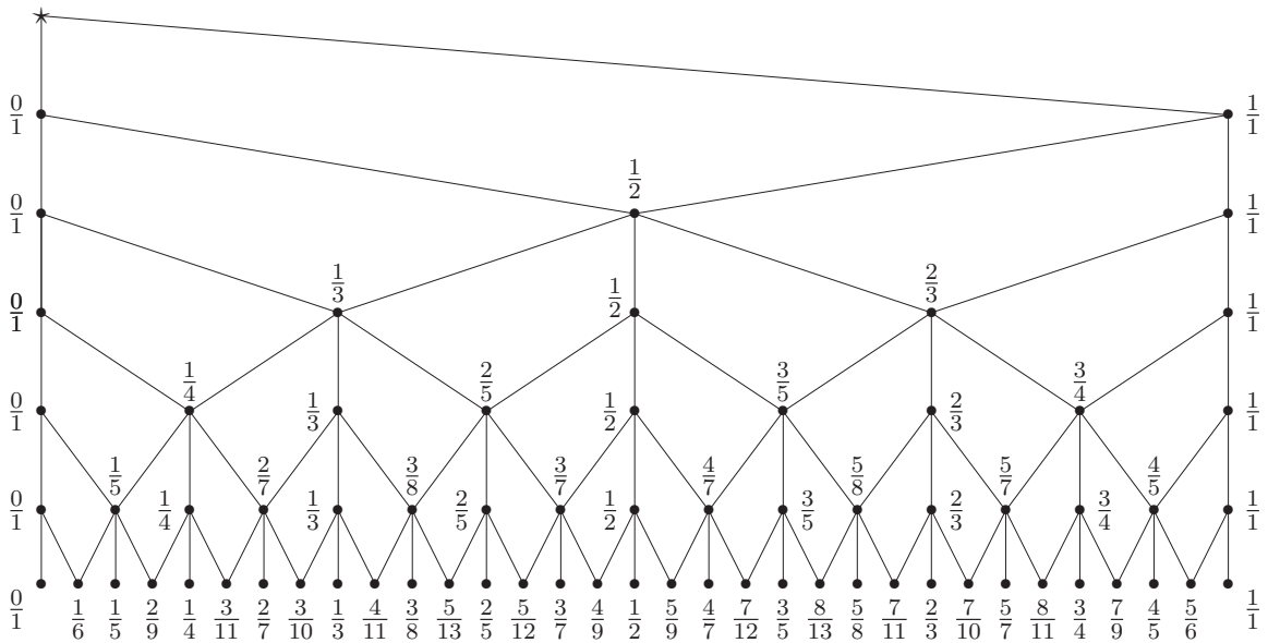
FIGURE 1. Bratteli diagram of \mathfrak{A}
