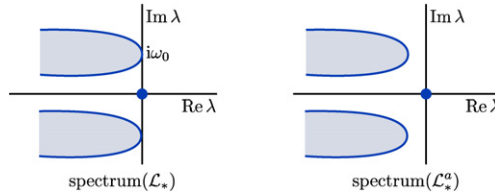
Fig. 2. The rightmost parts of the L^2_{ul} spectra of the linearization \mathcal{L}_* and the weighted operator \mathcal{L}_*^a with 0 < a \ll 1 are shown for the case where Hypothesis (H2) is met. Note that \omega_0 = k_0 c_* > 0 at Turing bifurcations.
