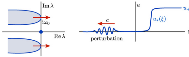
Fig. 1. The left panel illustrates the rightmost spectrum of the linearization about the front in the comoving frame \xi = x - ct at \mu = 0 . As \mu increases, we assume that essential spectrum crosses into the right half plane. The right panel illustrates how perturbations to the front profile are pushed, in the comoving frame, towards \xi = -\infty just after bifurcation, whilst their amplitude saturates at O(\sqrt{|\mu|}) .
